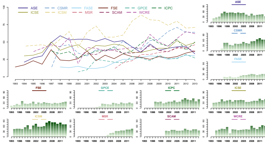
Figure 2: Variation of the number of programme committee members \#C(c, y) per year. Wide-scoped conferences (solid lines) have smaller PCs than narrow-scoped ones (dashed lines): p(\text{narrow}, \text{wide}) = 0.342^{**} . Relations between individual conferences are visualised in the \tilde{\mathbf{T}} -graph from Figure 4.
