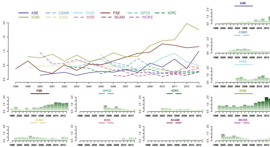
Figure 18: Variation of SR(c, y) —the average number of unsung heroes per PC member. Wide-scope conferences (solid lines) have more sustainable pools of PC candidates than narrow-scope ones (dashed lines): p(\text{narrow, wide}) = 0.762^{**} . Relations between individual conferences are visualised in Figure 19.
