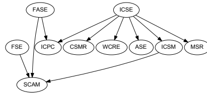
Figure 19: \tilde{\mathbf{T}} -graph for SR(c, y, 4) .
