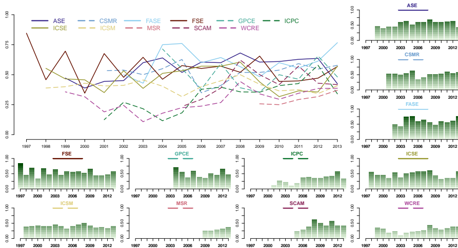
Figure 17: Variation of RCnA(c, y, 4) —the ratio of PC members for conference c in year y that have never co-authored a paper at any of the four preceding instances of c . The PCs of narrow-scope conferences (dashed lines) are more representative of their communities than those of wide-scope conferences (solid lines): p(\text{narrow}, \text{wide}) = 0.803^{**} . Relations between individual conferences are visualised in Figure 16.
