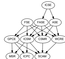
Figure 5: \tilde{\mathbf{T}} -graph for the review load \#RL .
