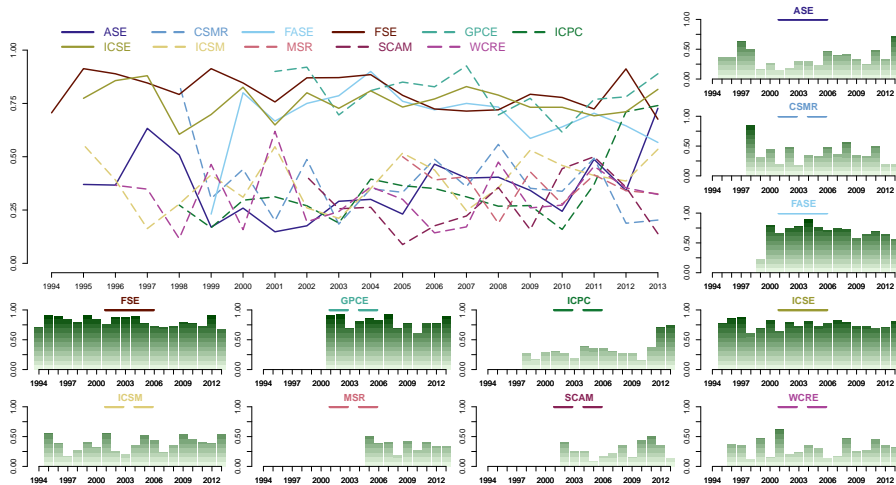
Figure 7: Variation of PC turnover w.r.t. previous year RNC(c, y, 1) . Wide-scoped conferences (solid lines) usually have higher values than narrow-scoped ones (dashed lines): p(\text{narrow, wide}) = 0.779^{**} . The \tilde{\mathbf{T}} -graph in Figure 8 confirms this, except for GPCE (which behaves like a wide-scoped conference) and ASE (which behaves like a narrow-scoped conference).
