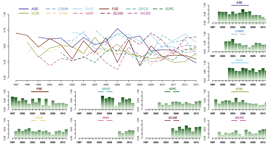
Figure 11: Variation of RPNA(c, y, 4) —the fraction of papers for which none of the co-authors has previously published at conference c in the 4 preceding years to y . Wide-scope conferences (solid lines) usually have higher values (are more open) than the narrow-scope ones (dashed lines): p(\text{narrow}, \text{wide}) = 0.627^{**} . Relations between individual conferences are visualised in Figure 13.
