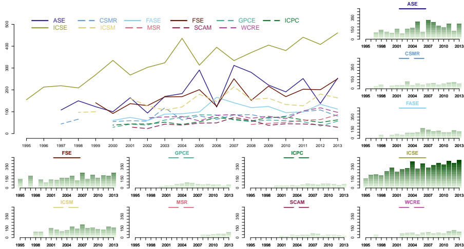
Figure 1: Variation of the number of submitted papers per year \#SP . “Gaps” correspond to older editions of the conferences, for which we could not retrieve the data. Wide-scoped conferences (solid lines) tend to receive more submissions than narrow-scoped ones (dashed lines): p(\text{narrow}, \text{wide}) = 0.911^{**} . Relations between individual conferences are visualised in the \tilde{\mathbf{T}} -graph from Figure 3.
