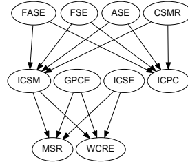
Figure 16: \tilde{\mathbf{T}} -graph for RCnA(c, y, 4) .
