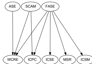
Figure 13: \tilde{\mathbf{T}} -graph for the ratio of papers by new authors w.r.t. four previous years RPNA(c, y, 4) . Statistically indistinguishable conferences are not displayed.
