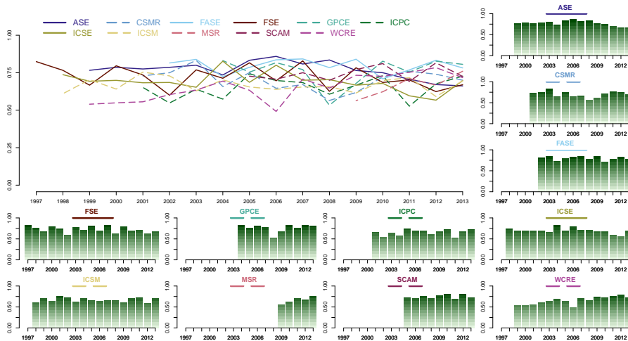
Figure 10: Variation of the author turnover w.r.t. four previous years RNA(c, y, 4) . Wide-scope conferences (solid lines) tend to have higher values than narrow-scope ones (dashed lines): p(\text{narrow}, \text{wide}) = 0.684^{**} . Relations between individual conferences are visualised in the \tilde{\mathbf{T}} -graph from Figure 9.
