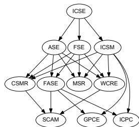
Figure 3: \tilde{\mathbf{T}} -graph for the number of submitted papers \#SP .
