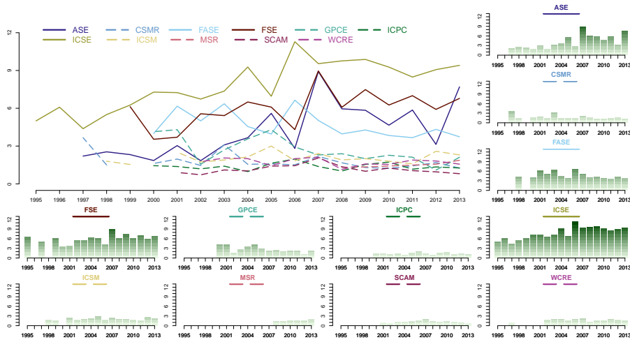
Figure 6: Variation of the review load RL per year. Wide-scoped conferences (solid lines) have higher review load than narrow-scoped ones (dashed lines): p(\text{narrow,wide}) = 0.973^{**} . Relations between individual conferences are visualised in the \tilde{\mathbf{T}} -graph from Figure 5.
