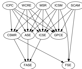
Figure 14: \tilde{\mathbf{T}} -graph for the ratio of papers co-authored by PC members in the same year RAC(c, y, \theta) .
