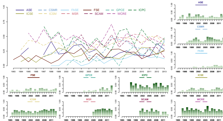
Figure 12: Variation of RAC(c, y, 0) —the fraction of papers co-authored by PC members in the same year. Wide-scope conferences (solid lines) tend to have lower values (are less introvert) than the narrow-scope ones (dashed lines): p(\text{narrow}, \text{wide}) = 0.144^{**} . Relations between individual conferences are visualised in Figure 14.
