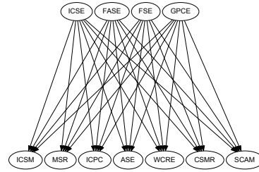
Figure 8: \tilde{\mathbf{T}} -graph for the PC turnover w.r.t. previous year RNC(c, y, 1) .
