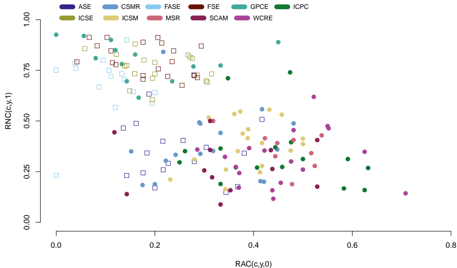
Figure 15: For narrow-scoped (filled circles) rather than wide-scoped (empty squares) conferences, higher PC turnover is associated with smaller fractions of PC papers among the accepted papers.
