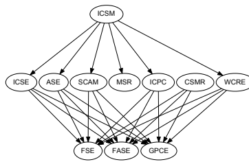
Figure 4: \tilde{\mathbf{T}} -graph for the number of PC members \#C .
