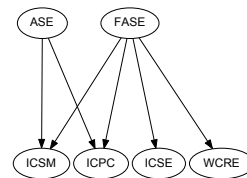
Figure 9: \tilde{\mathbf{T}} -graph for the author turnover w.r.t. four previous years RNA(c, y, 4) . Statistically indistinguishable conferences are not displayed.
